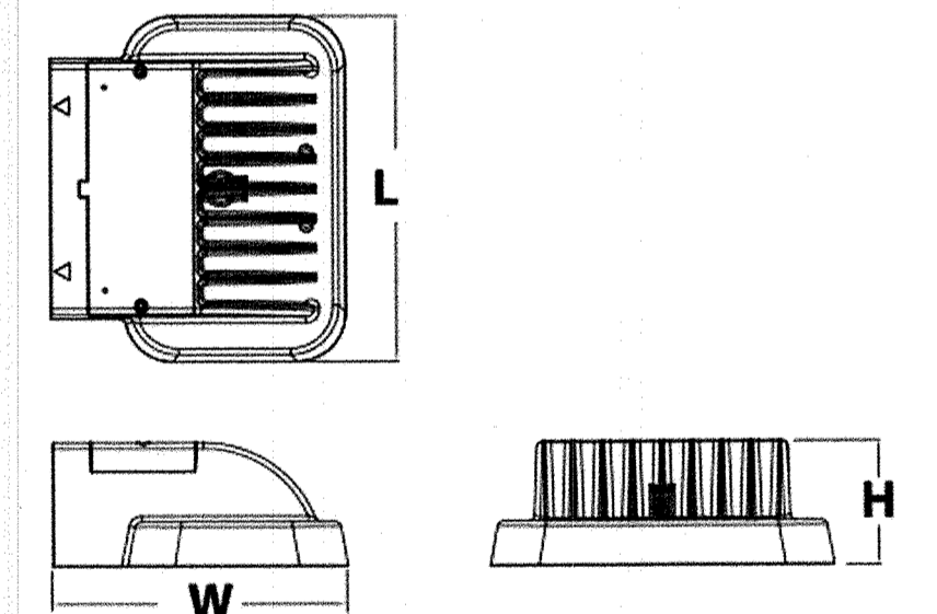
B LITHONIA KAXW-LED WALL PACK NOT TO SCALE
