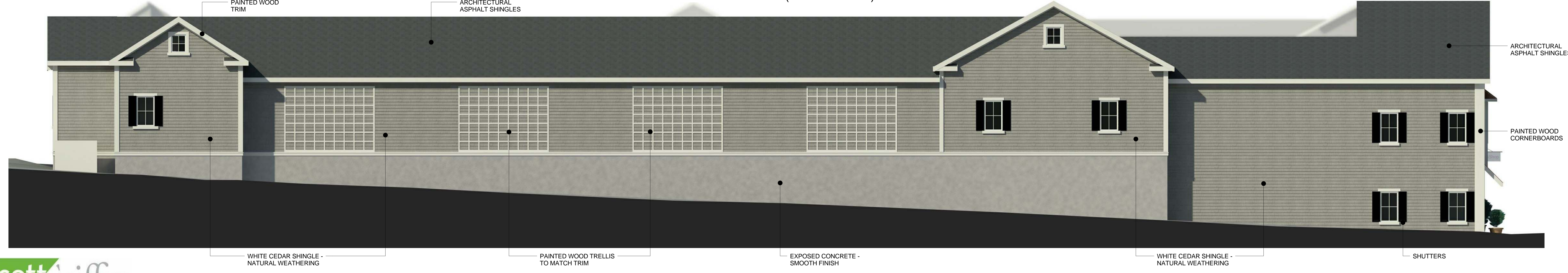
SOUTH ELEVATION
