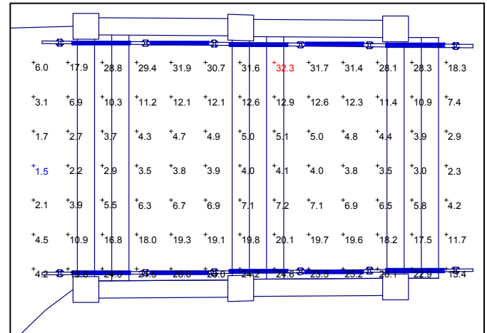
Photometric Layout
