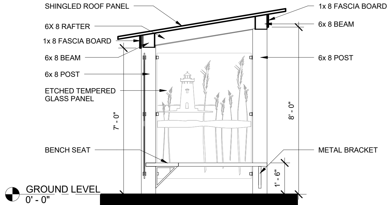
3 SECTION 3/8" = 1'-0"
