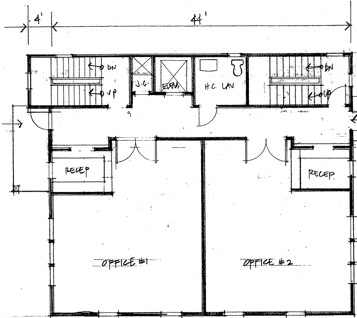
FIRST & SECOND FLOOR
