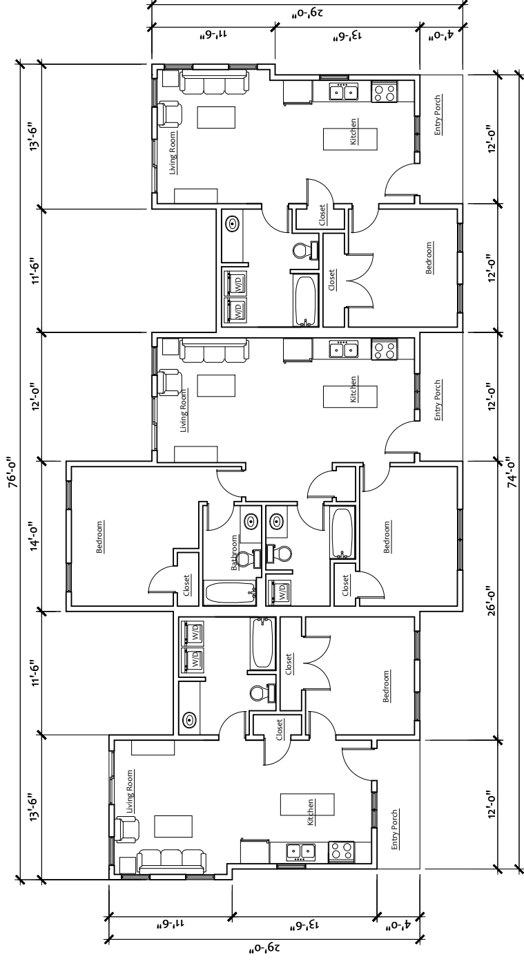
Preliminary TriPlex Floor Plan Scale: 1/8" = 1'-0"
