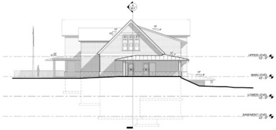
B WEST ELEVATION 3/8" = 1'-0"
