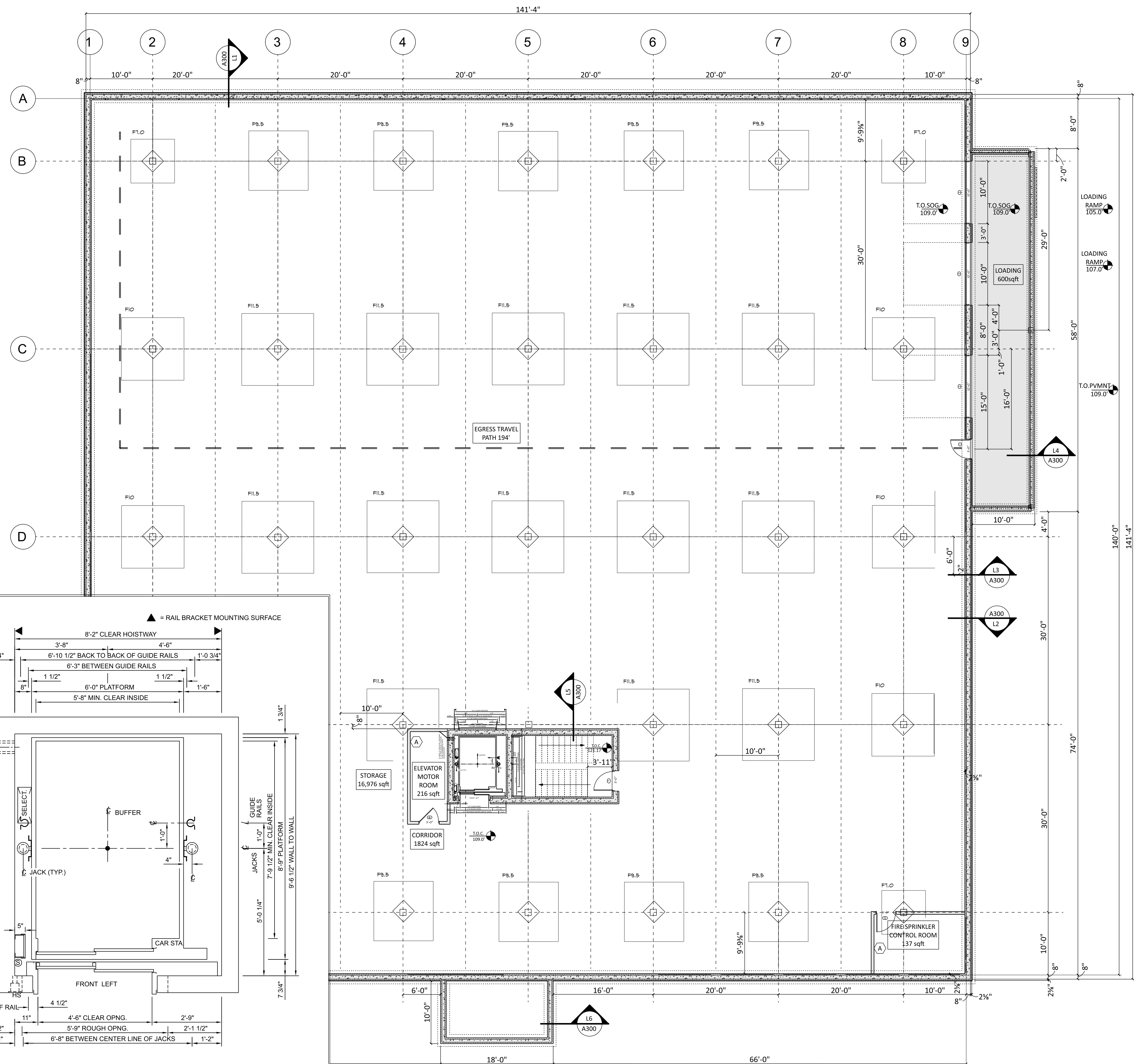
ELEVATOR DETAIL
