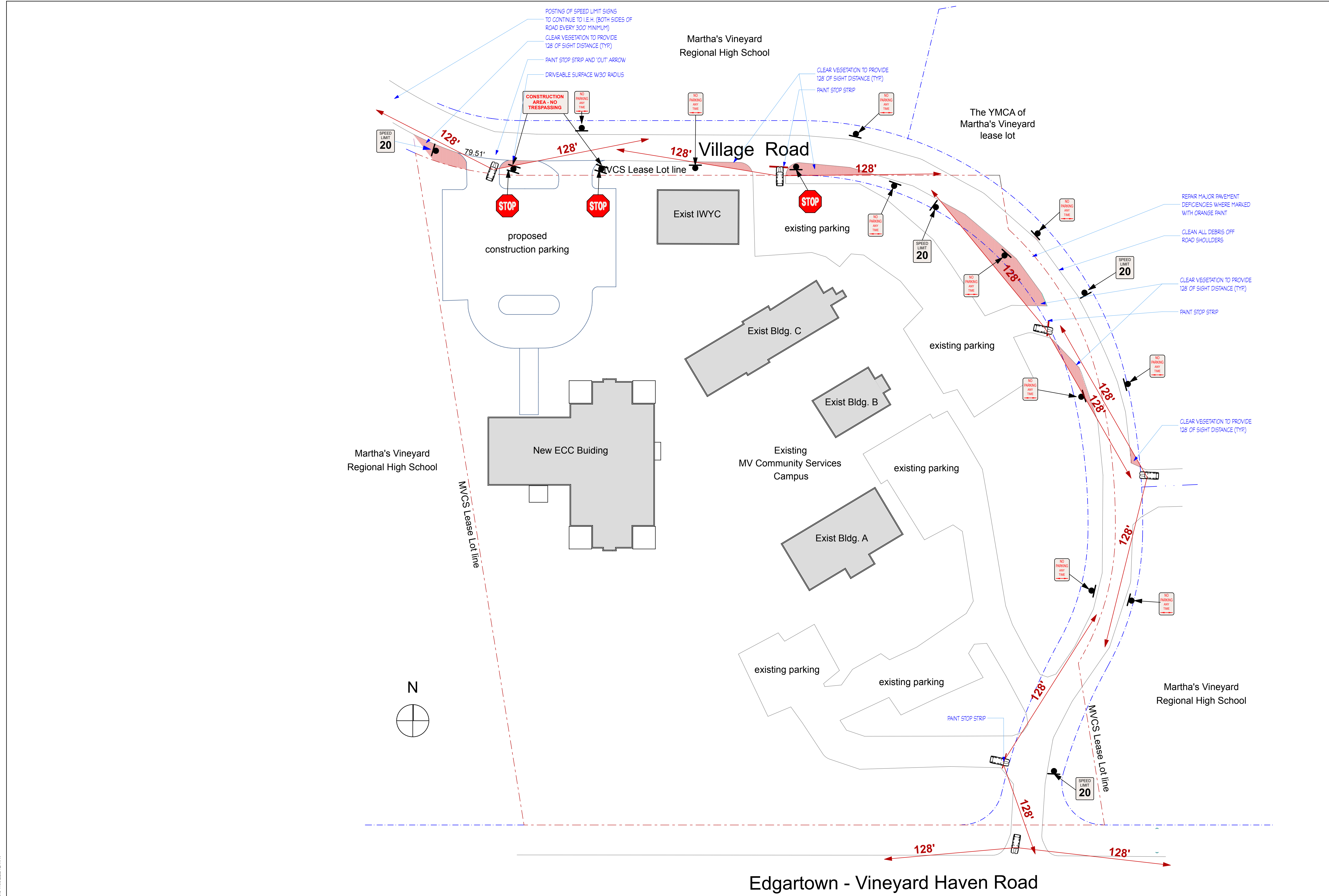
1 PHASE 1 VILLAGE ROAD IMPROVEMENT PLAN SCALE: 1" = 30'
