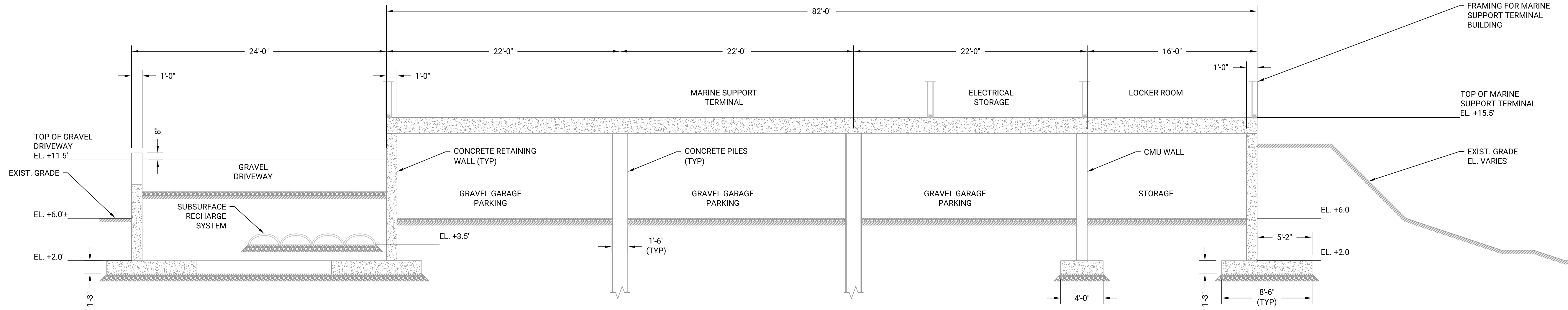
E-W SECTION THROUGH BUILDING SCALE: \frac{3}{16}'' = 1'-0''
