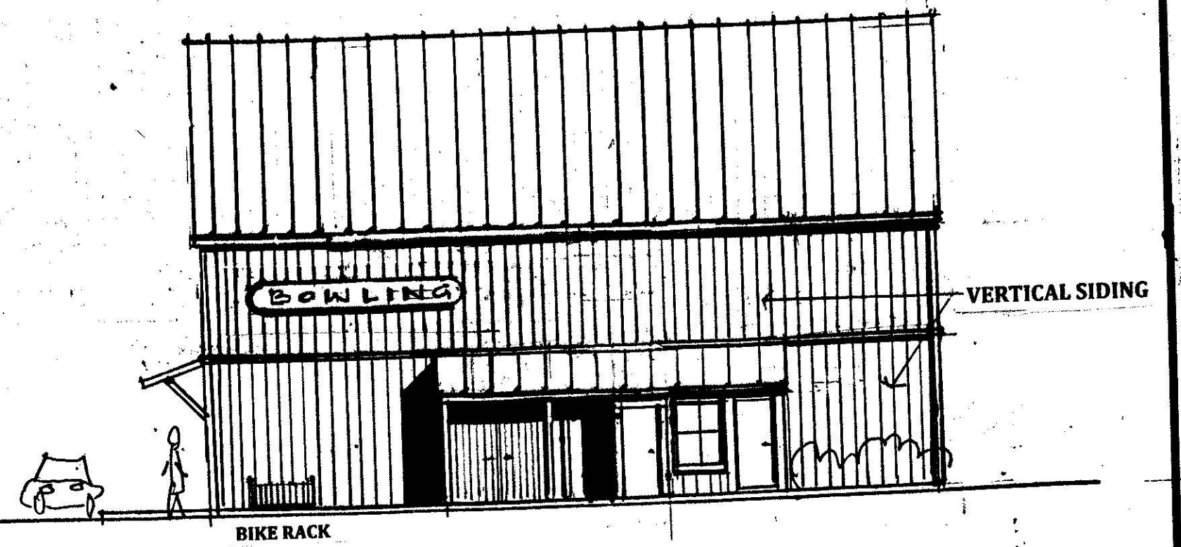
North Elevation 1"=10'
