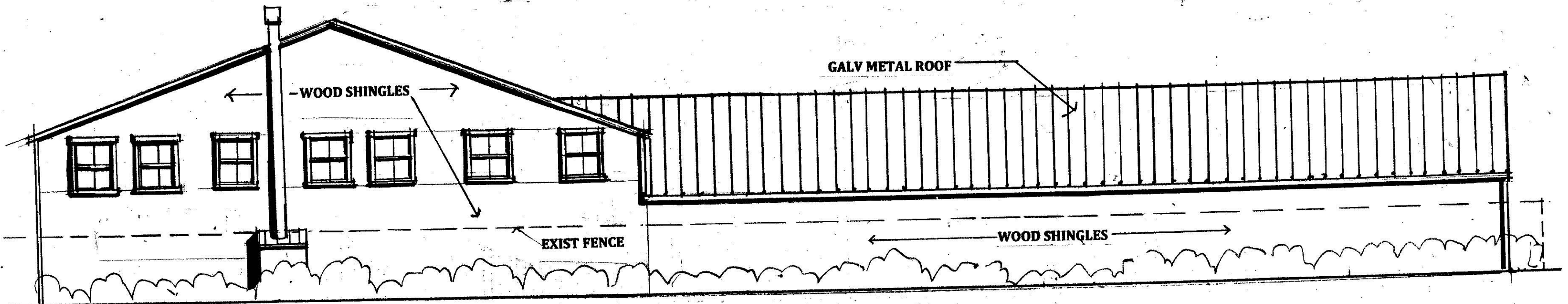
West Elevation 1"=10'
