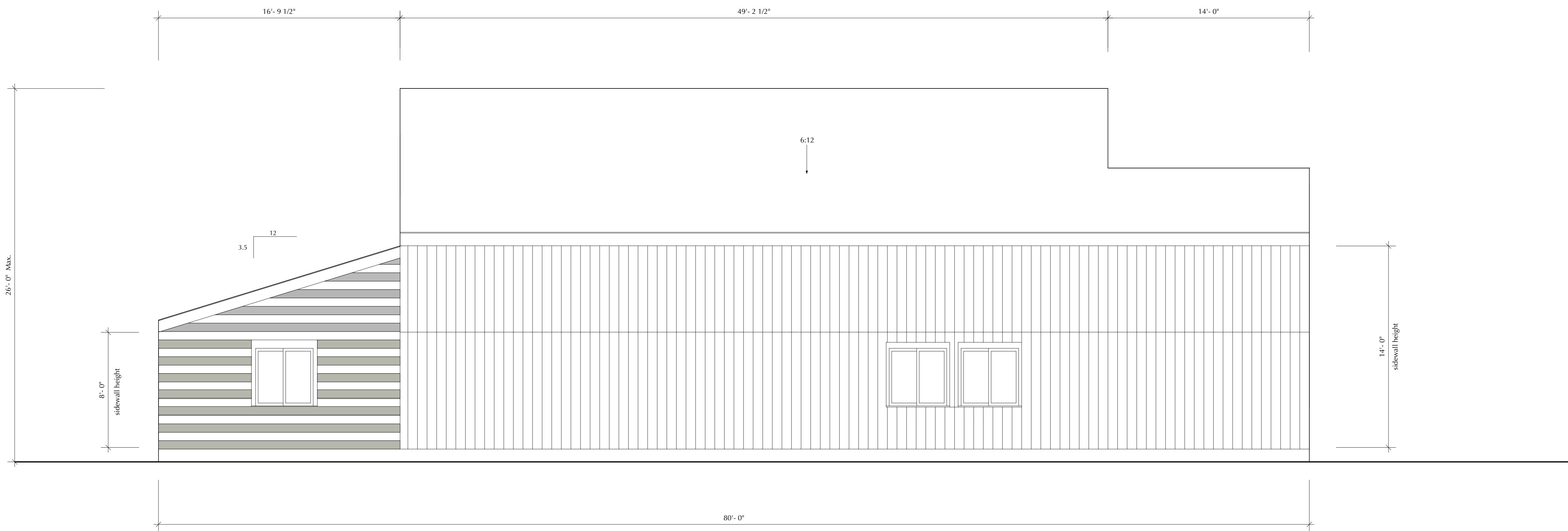
EAST ELEVATION
