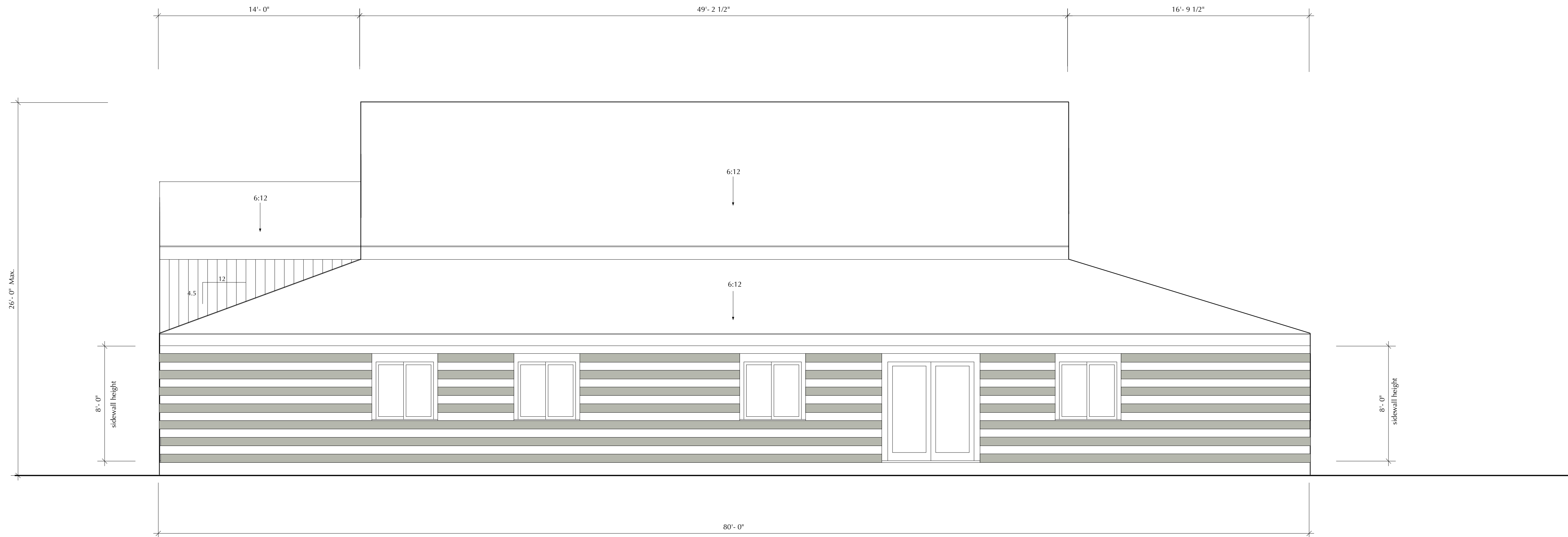
WEST ELEVATION
