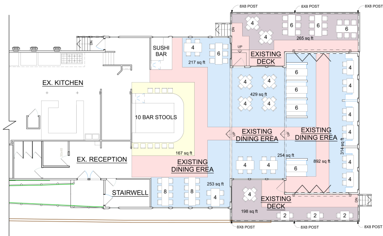
2015 FIRST FLOOR PLAN
