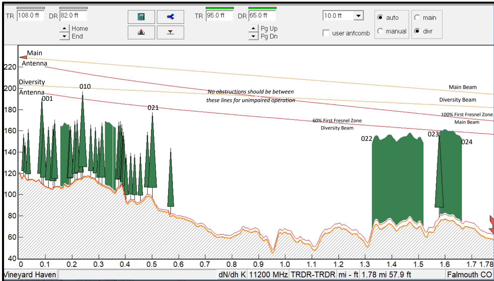
Vineyard Haven to Falmouth CO Path Profile (0 to 1.80 Miles) Main and Diversity Antennas Zoom from Pathloss 5 Software
