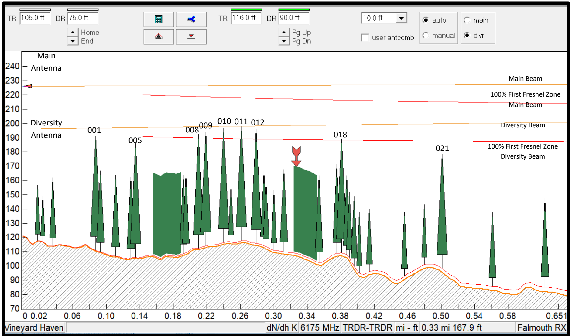
Vineyard Haven to Falmouth RX Path Profile (0 to 0.65 Miles) Main and Diversity Antennas Zoom from Pathloss 5 Software
