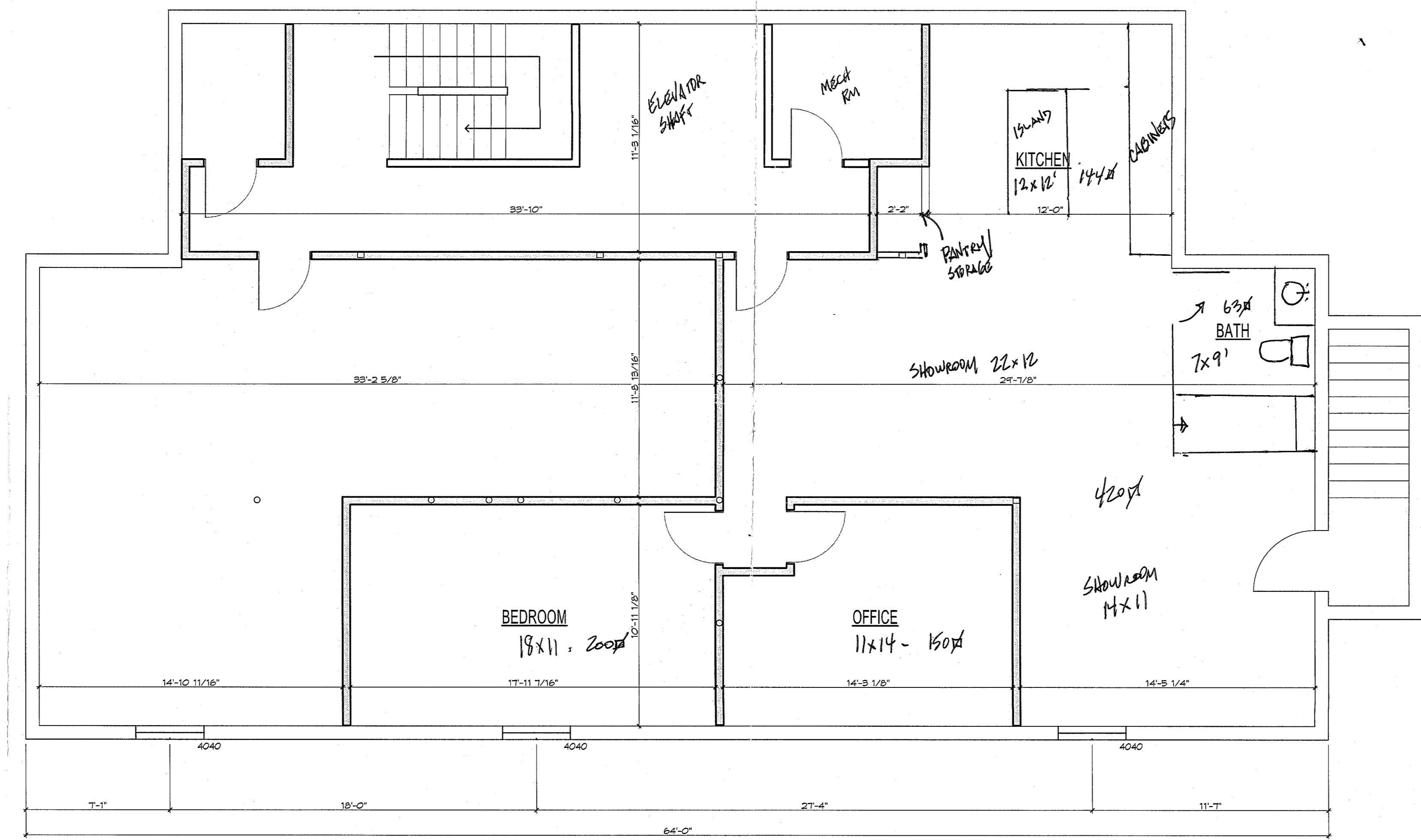
1 BASEMENT LAYOUT SCALE: 1/4" = 1'-0"
