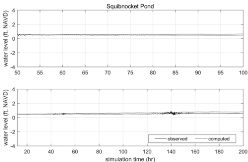
Figure V-14. Comparison of model output and measured tides for the TDR location at Squibnocket Pond at (MP5) for the final calibration model run (starting October 23, 2014 at 19:00 EST). The top plot is a 50-hour sub-section of the longer segment of the total modeled time period shown in the bottom plot.
