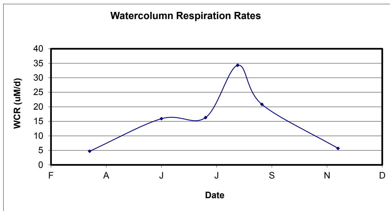
Figure VII-2. Average water column respiration rates (micro-Molar/day) from water collected throughout the Popponesset Bay System (Schlezingner and Howes, unpublished data). Rates vary ~7 fold from winter to summer as a result of variations in temperature and organic matter availability.
