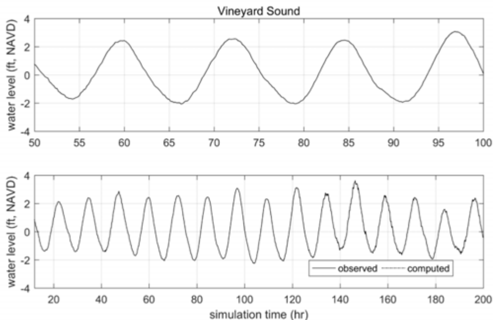
Figure V-10. Comparison of model output and measured tides for the TDR location offshore in Vineyard Sound (MP1) for the final calibration model run (starting October 23, 2014 at 19:00 EST). The top plot is a 50-hour sub-section of the longer segment of the total modeled time period shown in the bottom plot.
