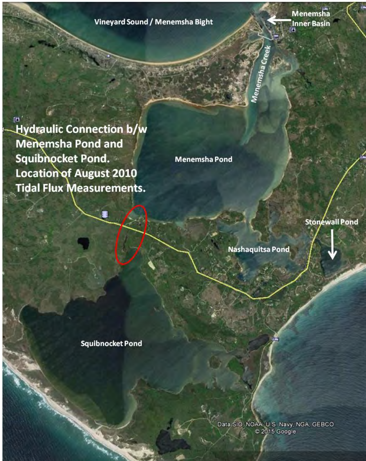
Figure IV-10 Menemsha Pond - Squibnocket Pond Embayment System. Red oval indicates the location of the herring run connecting the two basins. August 2010 tidal fluxes conducted at the culvert passing under the roadway.
